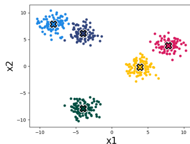
Figure 6.3: Converged result.
