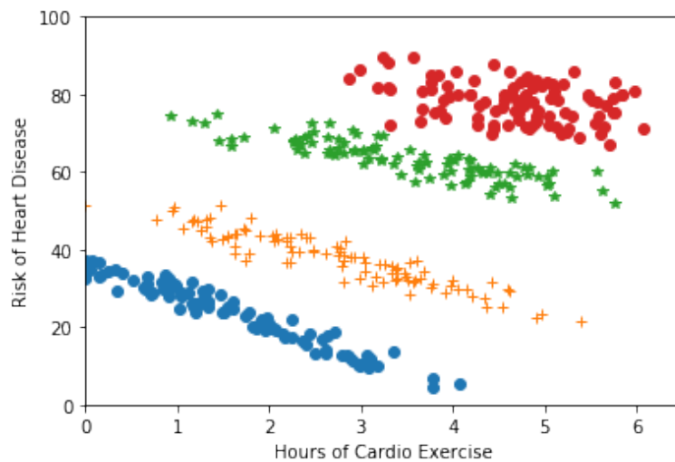
Figure 6.6: Averaged across the whole population, risk of heart disease positively correlates with hours of exercise. However, if we cluster the data, we can observe that there are four subgroups of the population which correspond to different age groups, and within each subgroup the correlation is negative. We can make better predictions, and better capture the presumed true effect, if we cluster this data and then model the trend in each cluster separately.
