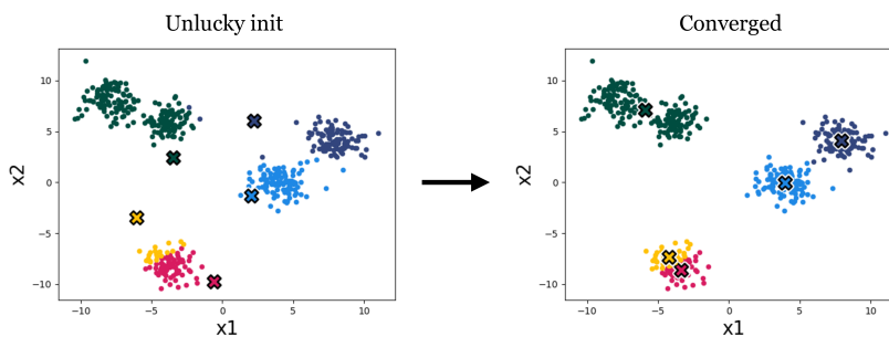
Figure 7.4: With the initialization of the means to the left, the yellow and red means end up splitting what perhaps should be one cluster in half.
