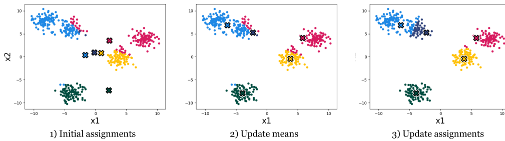
Figure 7.2: The first three steps of running the k-means algorithm on this data. Datapoints are colored according to the cluster to which they are assigned. Cluster means are the larger X's with black outlines.
